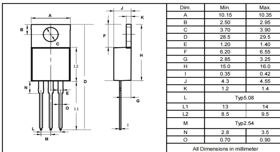
TO-220F
